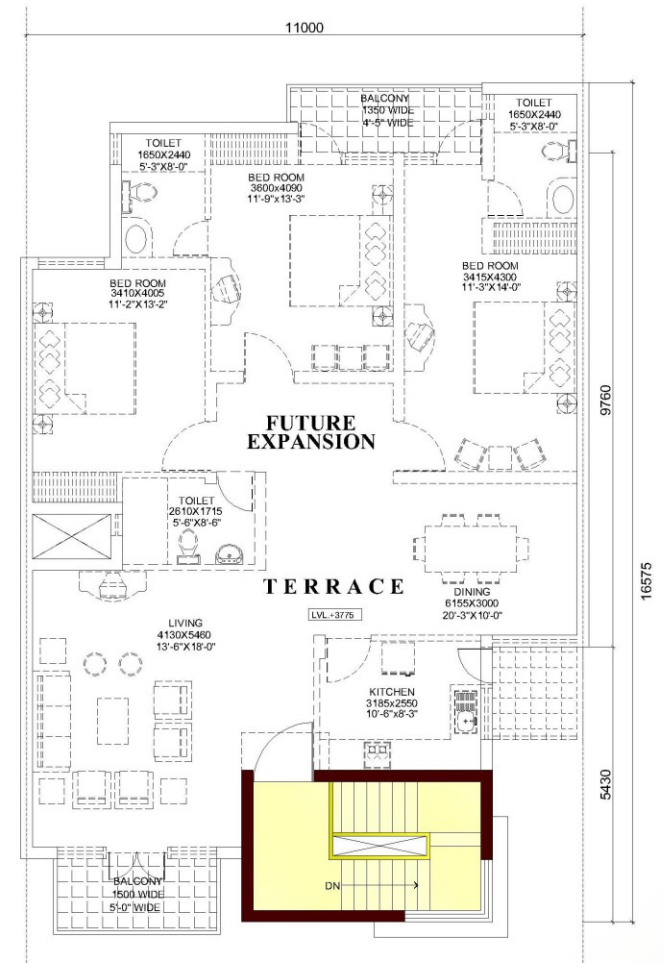
TERRACE PLAN
